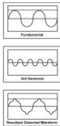
Figur 5: Sammansatt kurvform.
